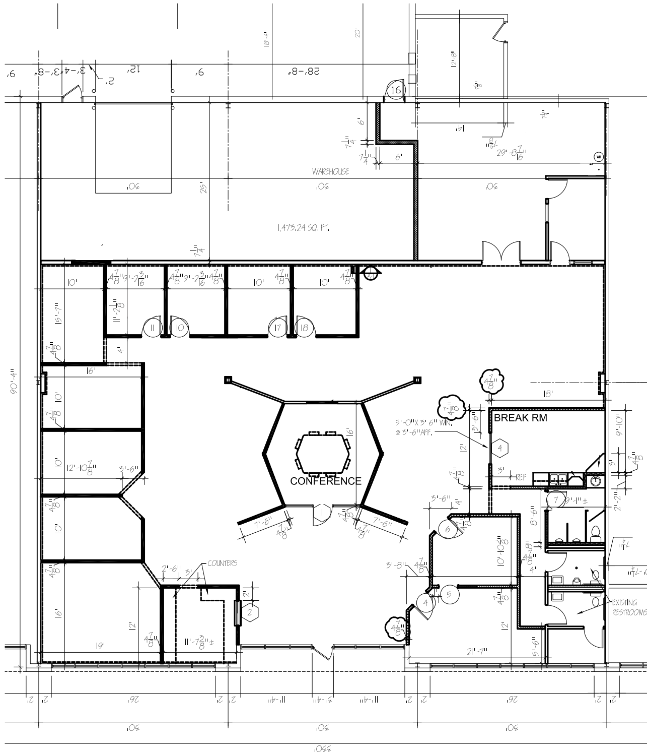
4 ENLARGED FLOOR PLAN 1/8" = 1'-0"
